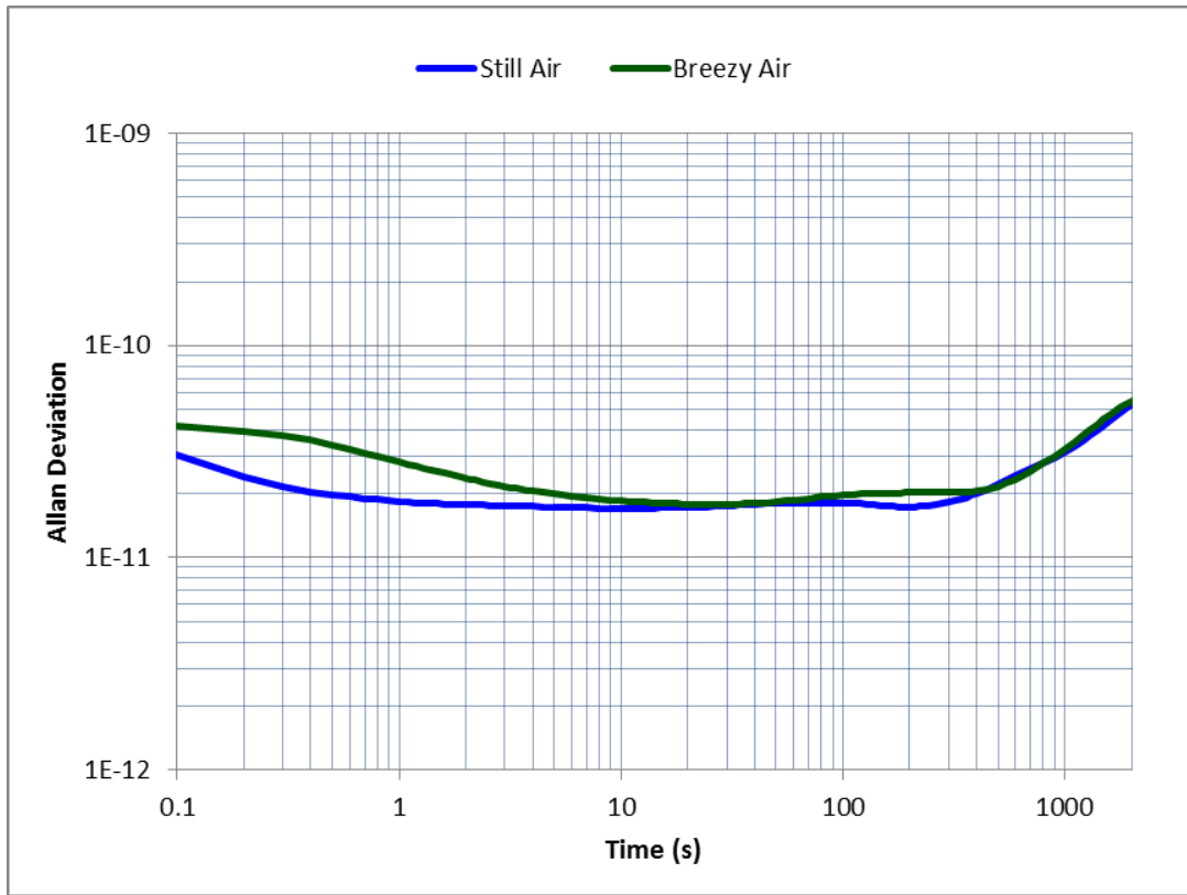
Figure 6: Allan deviation
