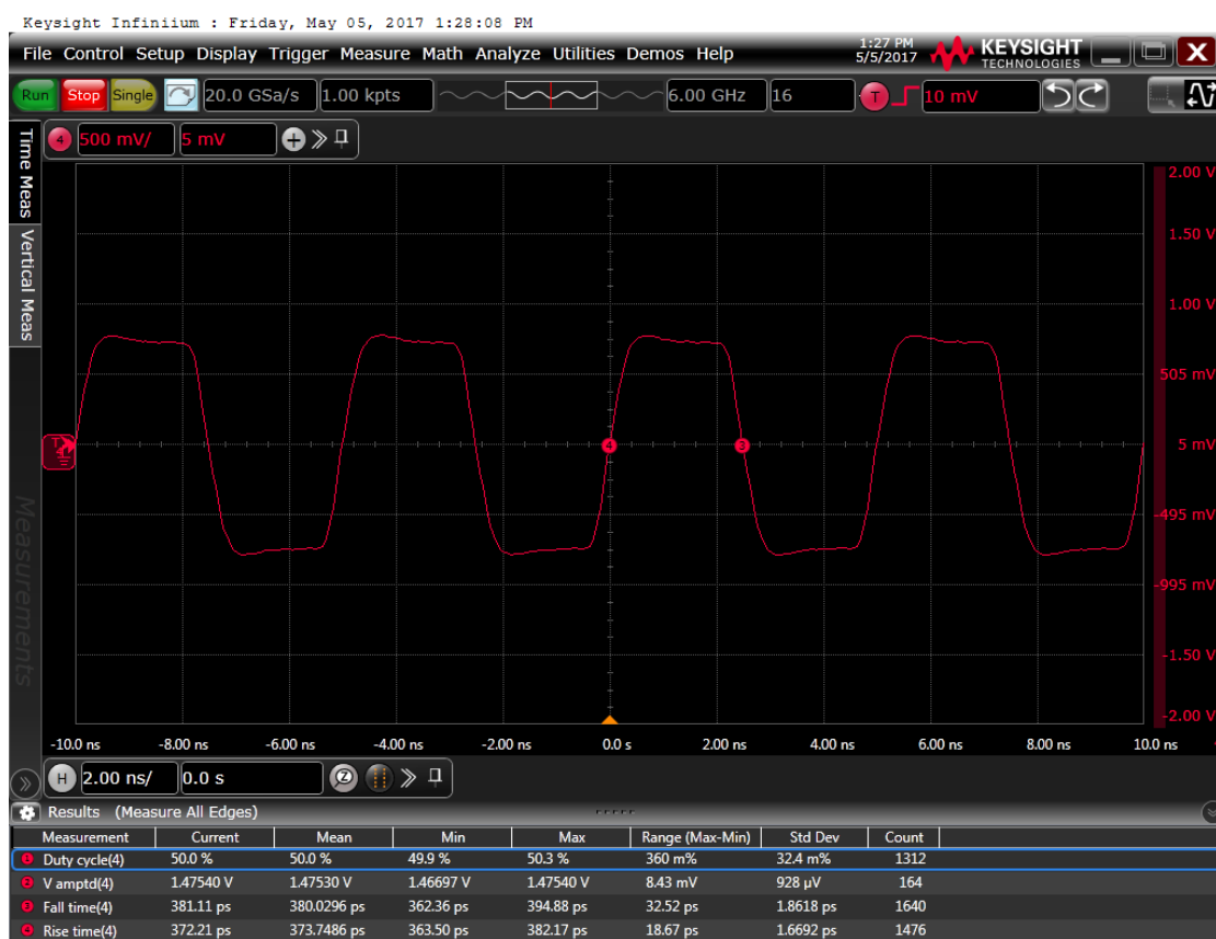
Figure 6: Output waveform, 2.5 V
