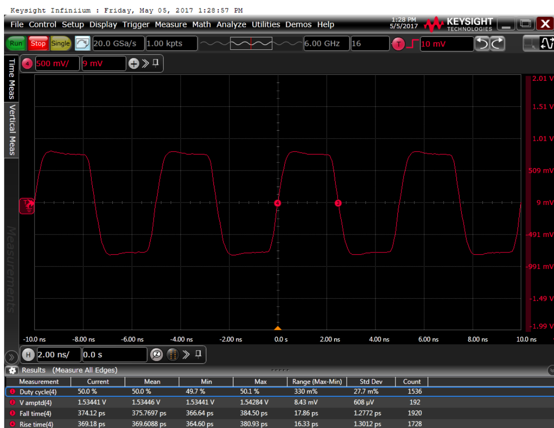
Figure 7: Output waveform, 3.3 V
