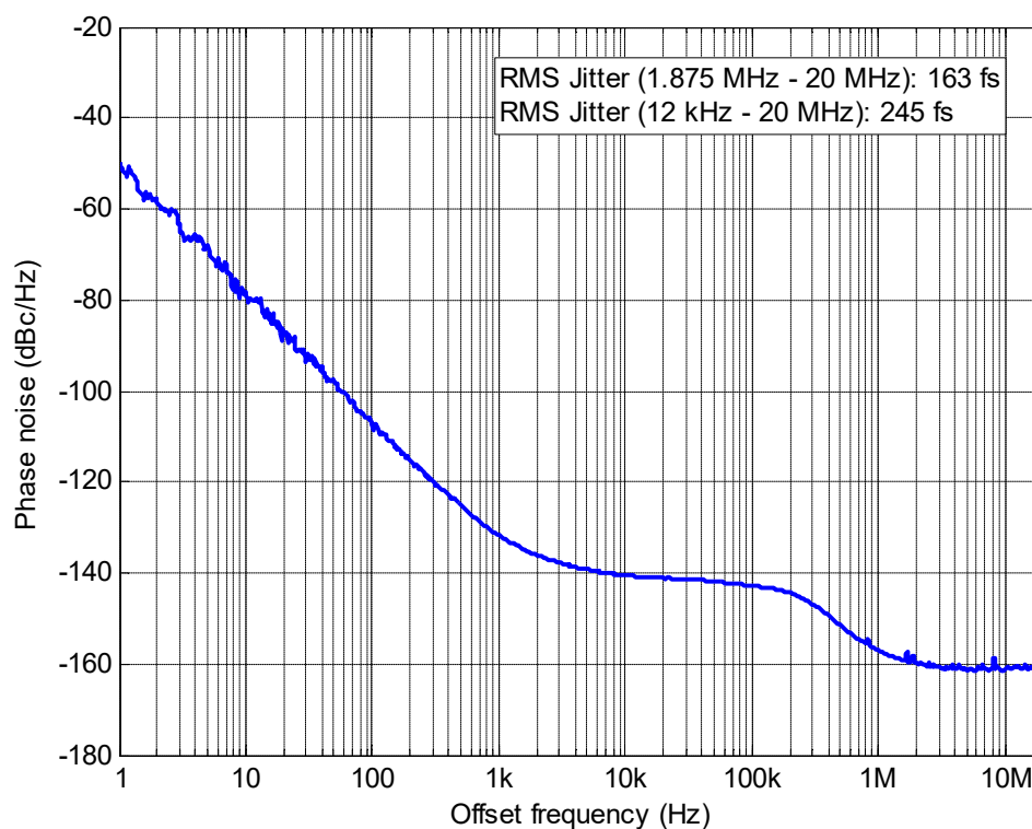
Figure 5: Phase noise, 3.3 V
