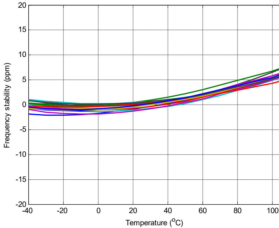
Figure 9: Frequency stability over temperature, 3.3 V
