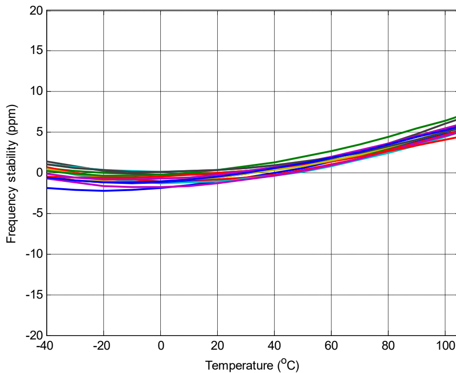
Figure 8: Frequency stability* over temperature, 2.5 V
